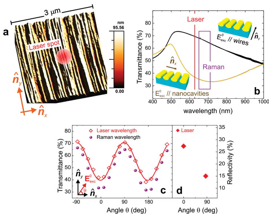
Figure 1. (a) AFM topography of the gold nanowire sample ( 3 \times 3 \mu\text{m}^2 ). The laser irradiated area (ca. 600 nm diameter) is indicated by the red spot. (b) Transmission spectra with excitation polarized parallel to the nanowires long axis \hat{n}_y (black line) or parallel to the wire-to-wire nanocavities axis \hat{n}_x (yellow line). The red line indicates the spectral position of the 633 nm laser line used for SERS; the violet box indicates the spectral range of the Raman scattering of MB molecules. (c) Sample transmittance at the laser (hollow red diamonds) and at the Raman wavelengths (violet solid circles) as a function of the angle \theta between the light polarization vector \hat{e}_{\text{exc}} and the wire-to-wire nanocavity axis \hat{n}_x . The red line is a fit of the transmittance using a T_0(1 - A \cos^2 \theta) model. (d) Sample reflectivity is higher (27%) for the field component along the nanocavity axis than for the one parallel to the nanowires long axis (15%).
